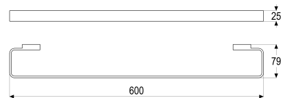
Dimensioned drawing
