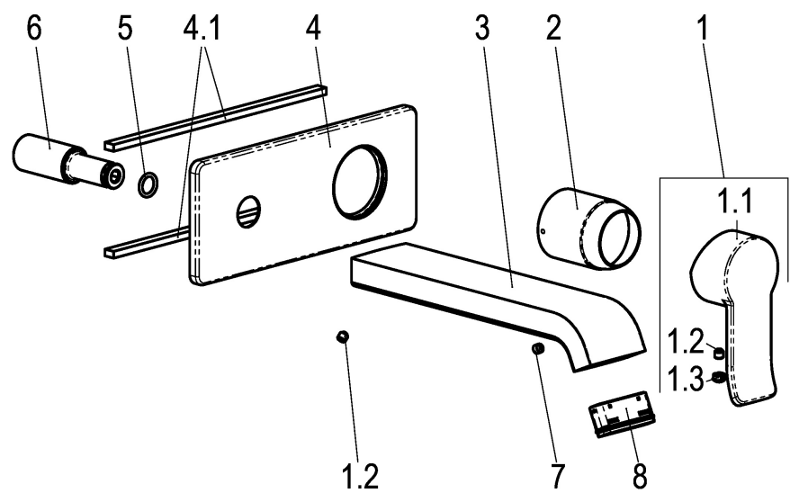
Exploded drawing
