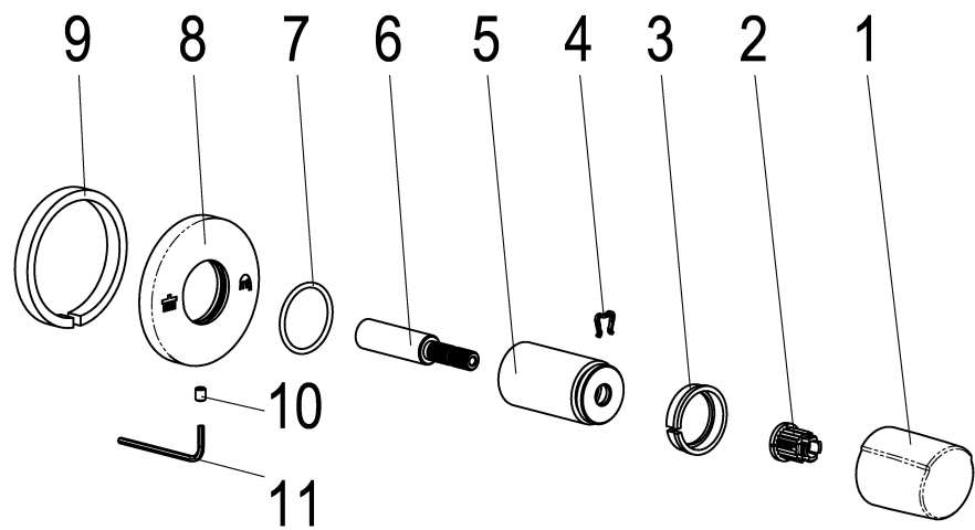
Exploded drawing
