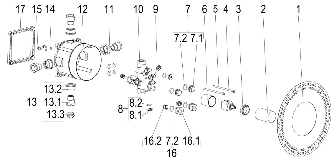
Exploded drawing
